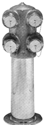
Figure No. 6540-6541 SQUARE STYLE
